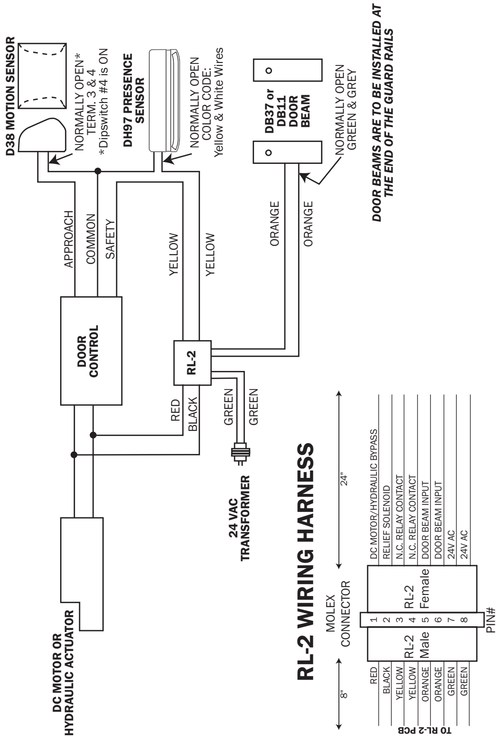
FIGURE 2 RL-2 SYSTEM WIRING DIAGRAM
