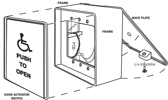
(Front View-Mounting Box Only)
